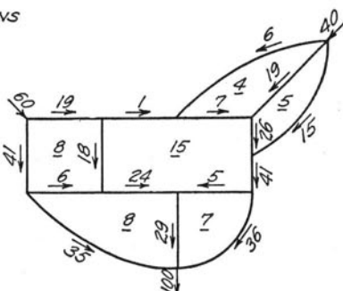
FIG. 3. DISTRIBUTION OF FLOW IN NETWORK—TWO INLETS; METHOD OF BALANCING HEADS
