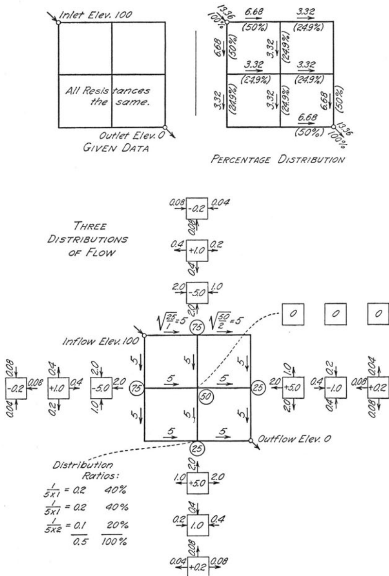
FIG. 6. DISTRIBUTION OF FLOW IN SIMPLE NETWORK; METHOD OF BALANCING FLOWS
