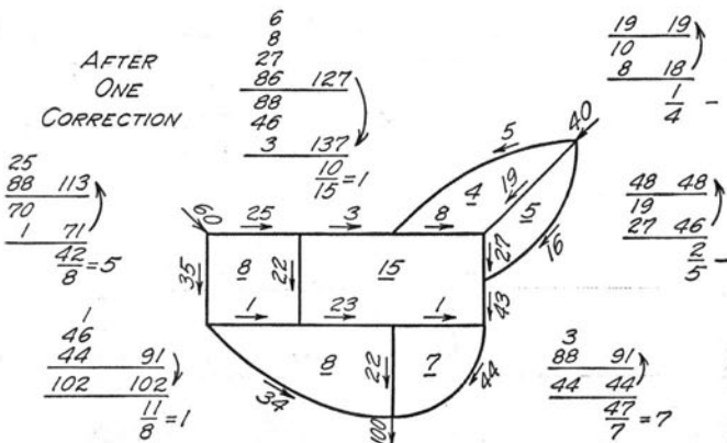
FIG. 3. DISTRIBUTION OF FLOW IN NETWORK—TWO INLETS; METHOD OF BALANCING HEADS
