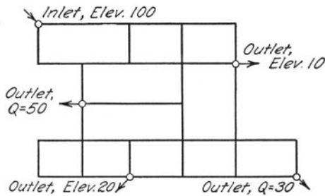
(e)-Several Outlets, Some Heads Fixed and Some Flows Fixed
