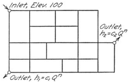
(d)-Several Outlets, Fixed Relation of Flow and Head
